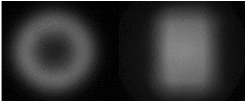
Figure 2 Left, Beam profile without diffuser. Right, Beam profile with rectangular diffuser.
