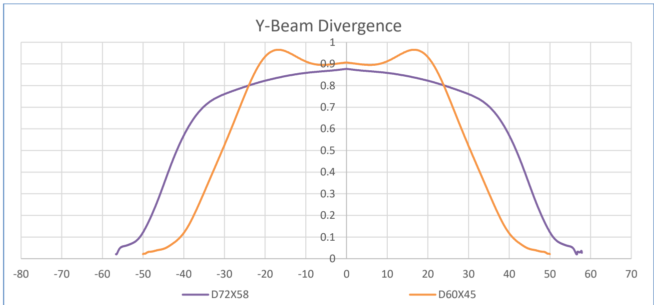
Figure 5 Y-direction beam divergence with their respective diffuser at 25°C, 1.5A. Operational Mode: 100µS, 10% Duty Cycle.
