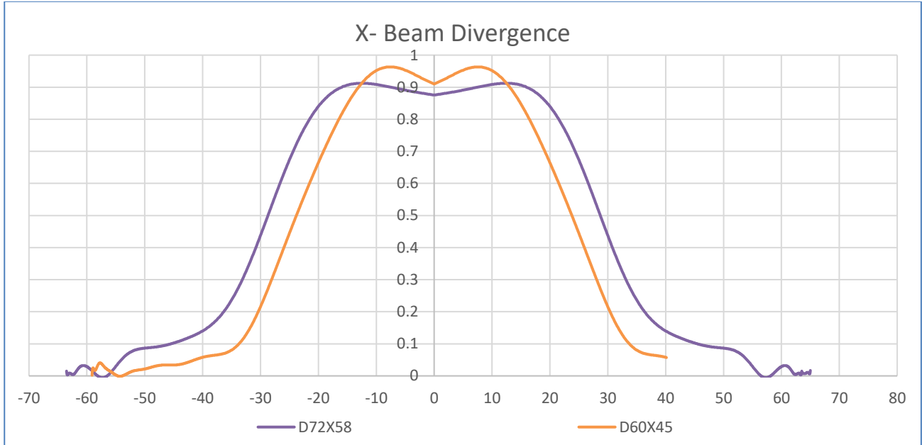
Figure 4 X-direction beam divergence with their respective diffuser at 25°C, 1.5A. Operational Mode: 100µS, 10% Duty Cycle.
