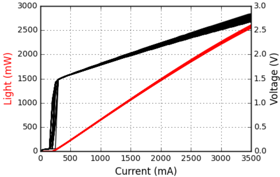
Figure 3 I-V data are a 2-point measurement, actual VCSEL forward voltage is lower. Operational mode: 100 \mu S, 1% Duty Cycle at 40°C.
