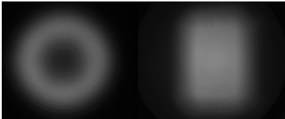
Figure 2 Left, Beam profile without diffuser. Right, Beam profile with rectangular diffuser.
