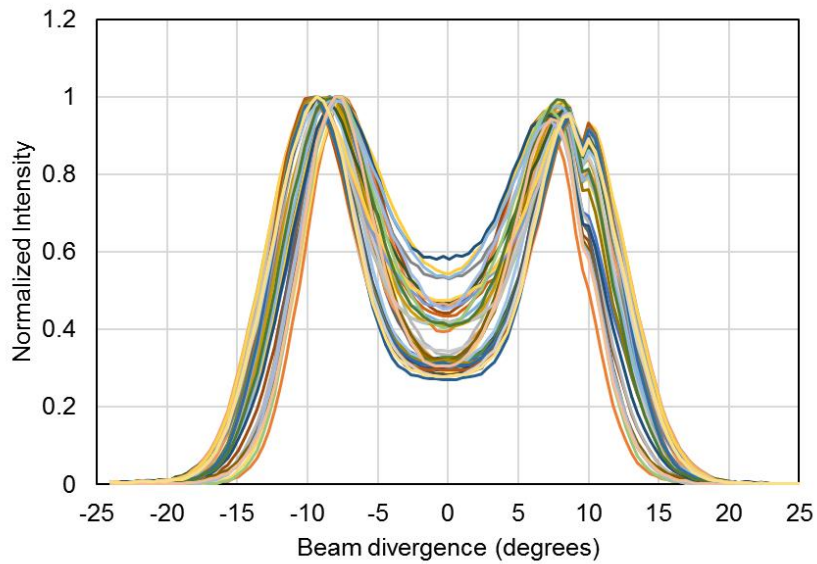
Figure 4 Beam Divergence of many VCSELs
