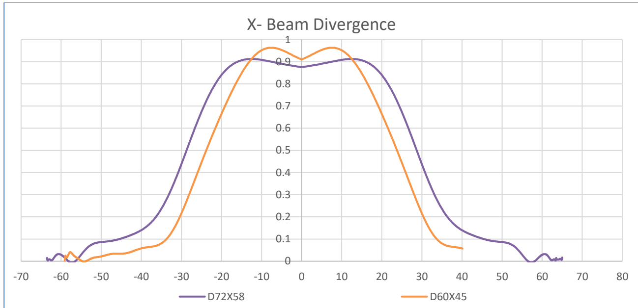
Figure 5 X-direction beam divergence with their respective diffuser at 25°C, 1.5A. Operational Mode: 100µS, 10% Duty Cycle.
