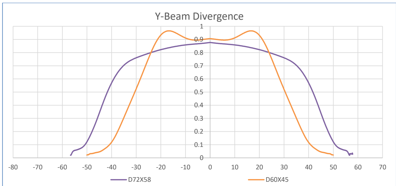
Figure 6 Y-direction beam divergence with their respective diffuser at 25°C, 1.5A. Operational Mode: 100µS, 10% Duty Cycle.
