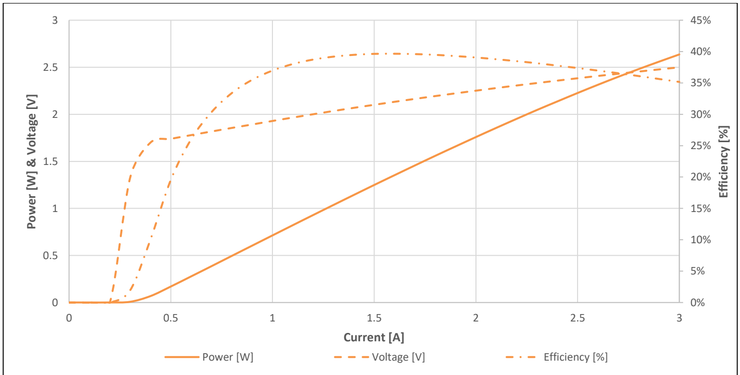
Figure 3 L-I-V of K0-0850M-0000-00041 at 100 \mu S, 10% Duty Cycle, 25°C
