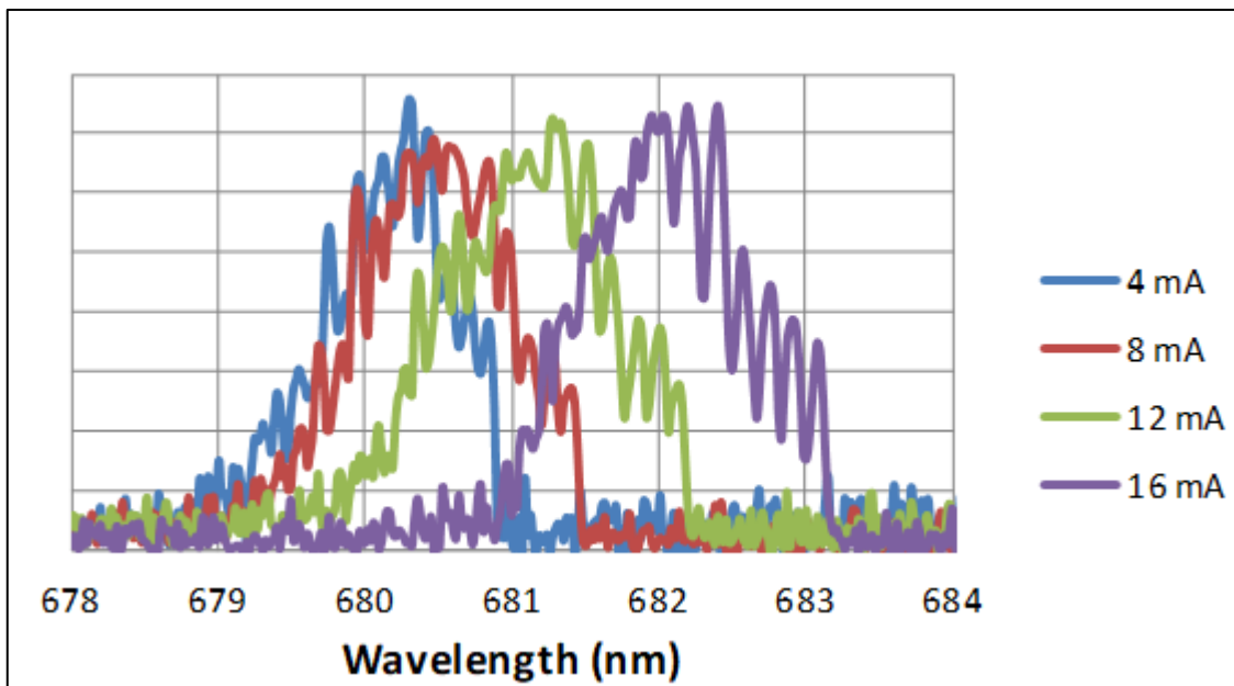
Figure 2 Spectral wavelength of I0-0680M-0000-X002 vs Current
