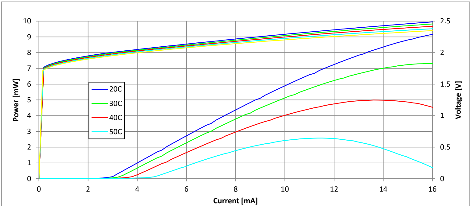
Figure 1 L-I-V of I0-0680M-0000-X002 vs Temperature
